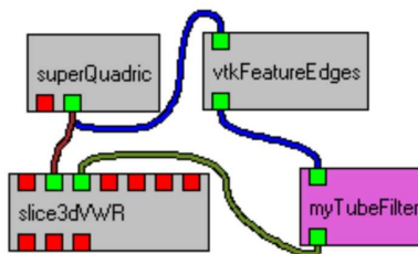
Figure 2.9: The DeVIDE network shown in figure 2.7 with the myTubeFilter module integrated.
