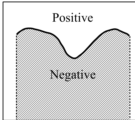
Figure 3.12: The signed distance field generated from the delineated curve. Above and to the sides the distance values are positive (i.e. the non-hatched areas)
