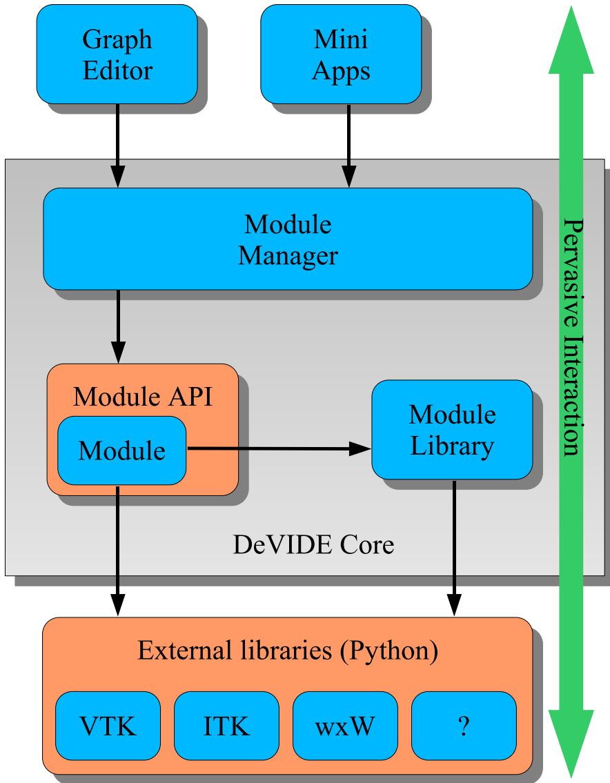
Figure 2.5: Diagram of the high-level DeVIDE architecture. The Module Manager is the main external interface.
