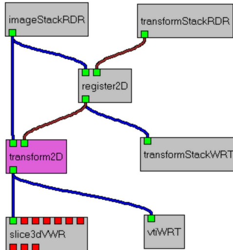
Figure 3.8: The DeVIDE modules and network that were used to perform the registration.
