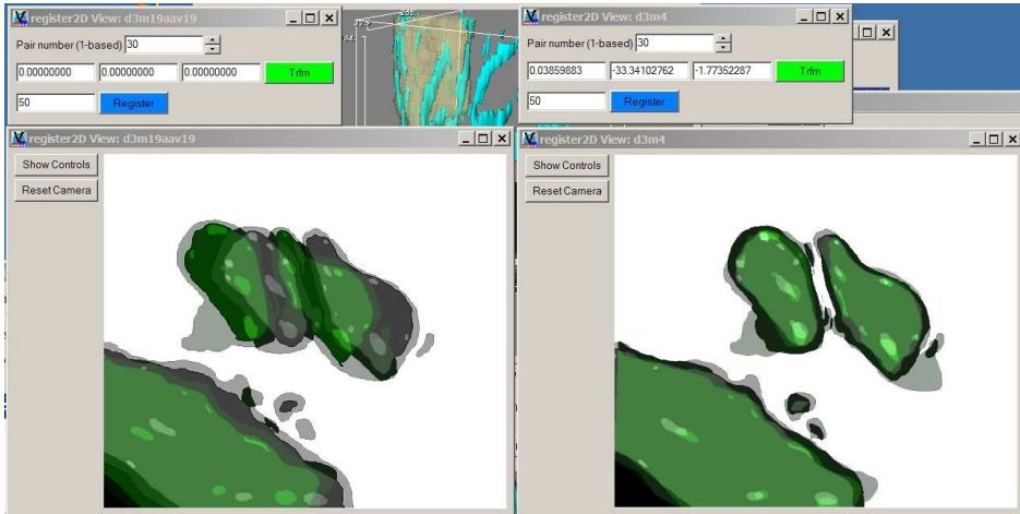
Figure 3.9: The user-interface of the register2d DeVIDE module.
