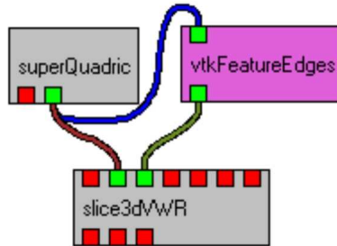
Figure 2.7: DeVIDE network that extracts different types of edges from a superquadric mesh. The mesh and the extracted edges are visualised together in the slice3dVWR module.
