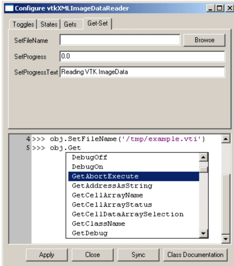
Figure 2.15: Screenshot of sample introspection session with a VTK object after it has been selected from the object drop-down list on the second to last row of the dialogue in figure 2.14.
