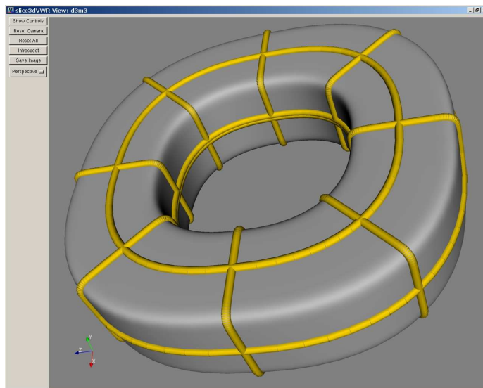
Figure 2.10: A visualisation that makes use of the newly-created myTubeFilter module to emphasise discontinuities in the sample mesh.
