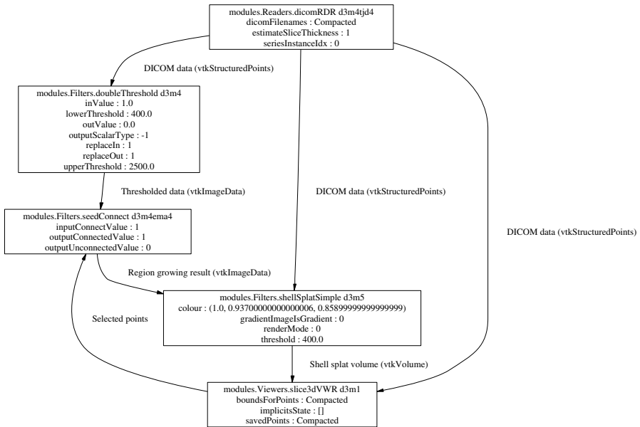
Figure 2.3: Alternative representation of the simple network shown in figure 2.2. All explicit algorithm parameters are also shown: this is useful when documenting experiments.
