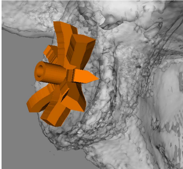
Figure 3.5: An earlier mould design that is in the process of being constructed by DeVIDE according to a set procedure, the patient-specific scapular surface and the final pre-operative planning parameters.
