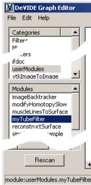
Figure 2.8: The Graph Editor’s module palette (shortened) showing the module categories at the top, with the userModules category selected. Modules in the currently selected categories are shown in the bottom list. A module can belong to more than one category. Multiple categories can be selected.
