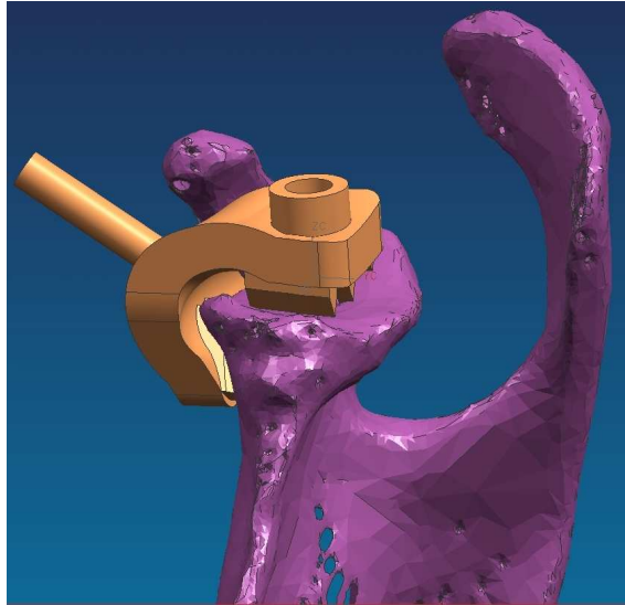
Figure 3.4: The latest design of the glenoid drill guide visualised on a surface model of a scapula. Illustration courtesy of Liesbet Goossens and Bart de Schouwer, Katholieke Universiteit Leuven, Belgium.
