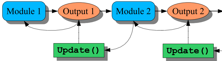
Figure 2.12: The DeVIDE demand-driven execution model. Due to the simple update convention, output data update requests propagate backwards through any given network until the source module is reached. Processing then propagates forwards until it reaches the final output object.
